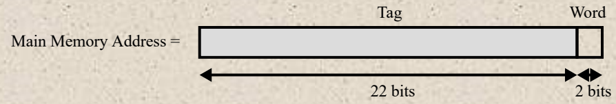
Figure 4.12 Associative Mapping Example
