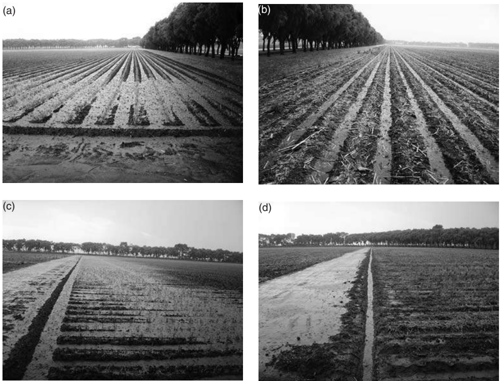
Fig. 10.6. The result of a severe rainfall event (30 mm in ~1 h) in a conventionally tilled field (a and c) and an adjacent conservation agriculture field with permanent raised beds and crop residue retained on the soil surface (b and d) in the CIMMYT high rainfall humid (2640 m above sea level; 19.17°N, 99.33°W silty clay loam soil of volcanic origin) experiment station in the central highlands of Mexico (photographs courtesy of F. Delgado).
