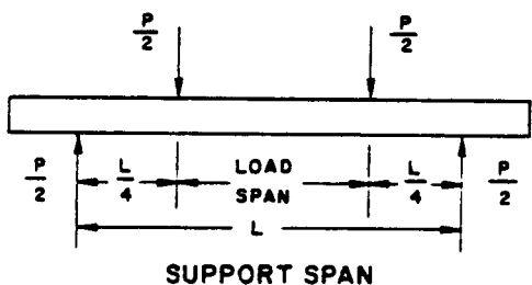
(one half of support span)
